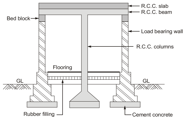
Composite Structure
