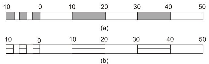
Fig. 1.1 Graphical scale
