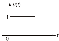
u(t) (Unit step function) (i)
