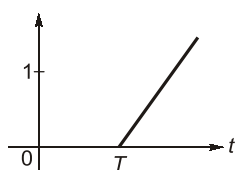
\frac{(t - T)}{T} u(t - T) (Right shifted unit ramp function) (iii)
