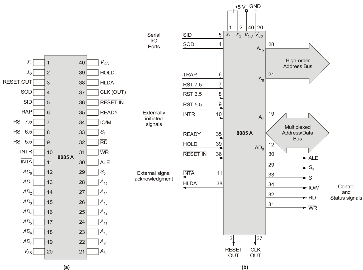
Figure-1.2 : 8085 Pinout
